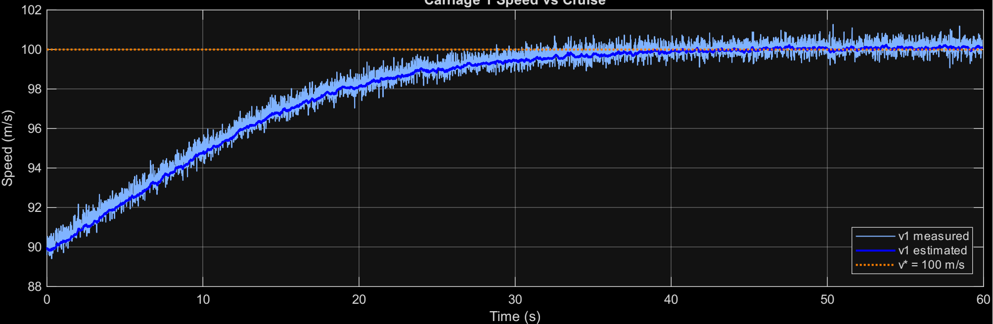
Carriage 1 Speed vs Cruise
