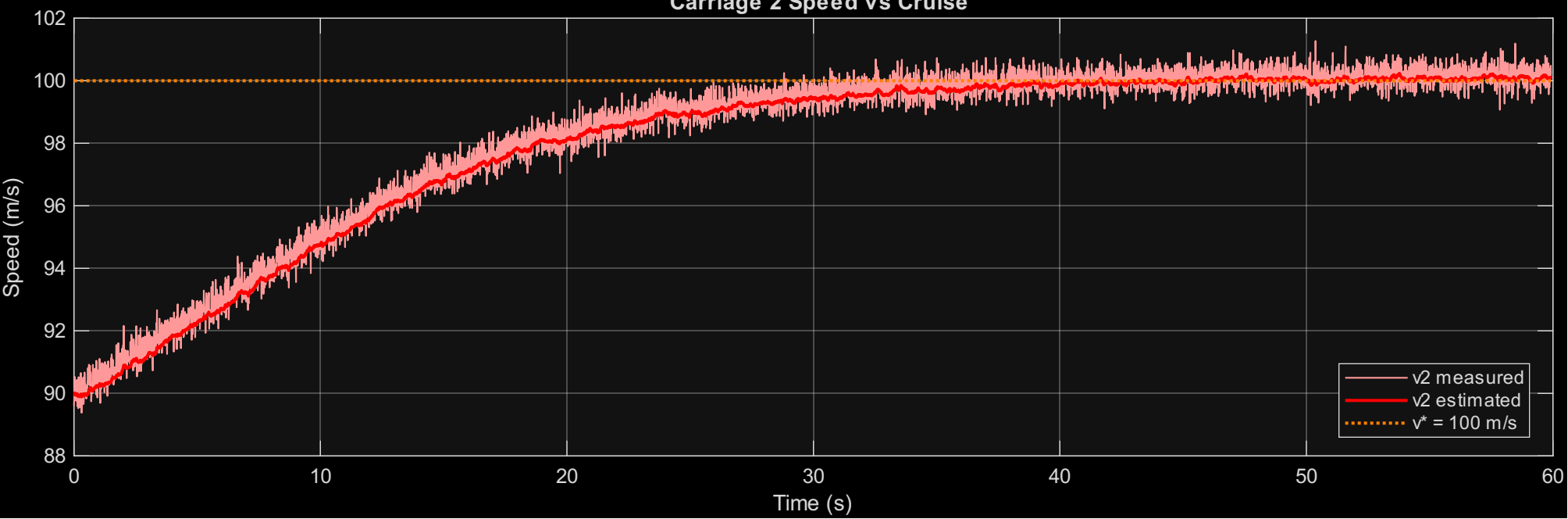
Carriage 2 Speed vs Cruise
